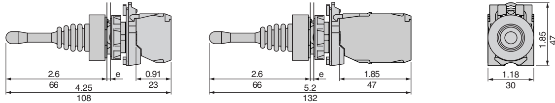
Joystick controllers XD5PA•2
