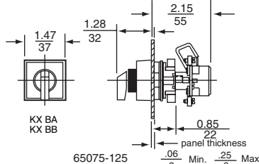
Single Pot Potentiometer Operator
