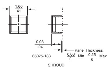
Shroud
