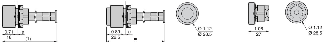
for potentiometer ZB5AD9•2
