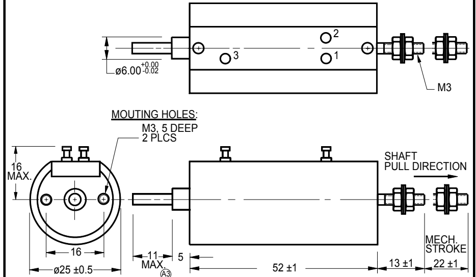
FIGURE 1 OUTLINE DIMENSIONS
