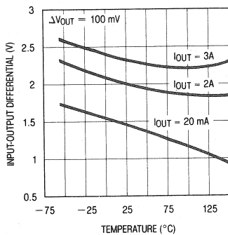
Dropout Voltage
