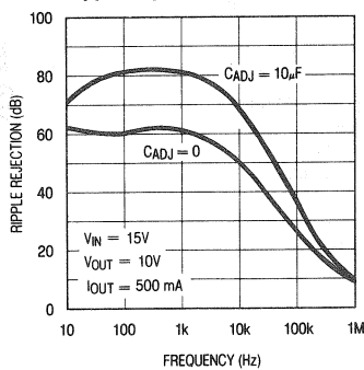
Ripple Rejection
