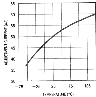
Adjustment Current
