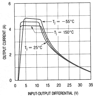
Current Limit
