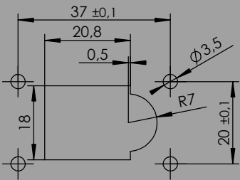
Hole pattern
