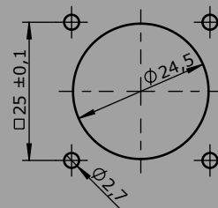
Hole pattern
