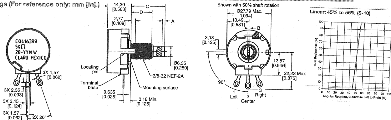
Dimensional Drawings (For reference only: mm [in.])
