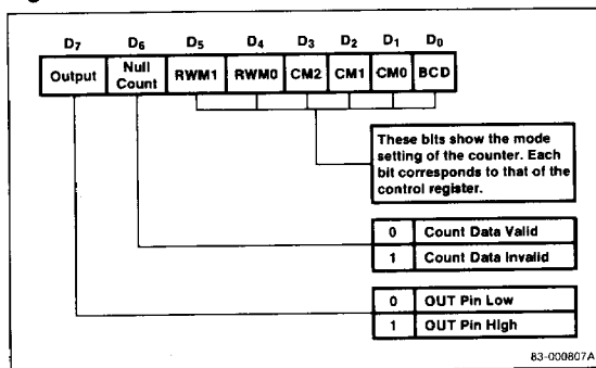
Figure 6. Status Data
