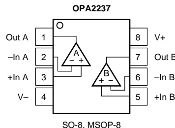
SO-8, MSOP-8
