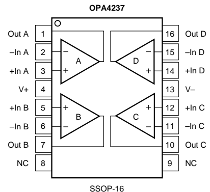
SSOP-16
