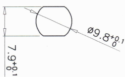
SUGGESTED PANEL CUTOUT
