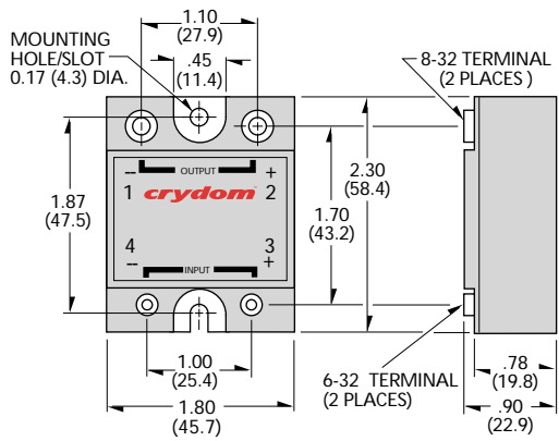
All dimensions are in inches (millimeters)
