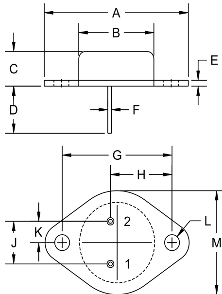
TO-3 50 mil
