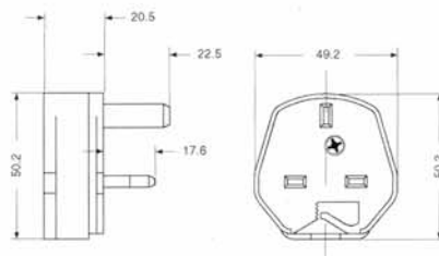
GB-Stecker
