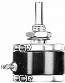
BUSHING MOUNT/SLEEVE BEARING MODEL 2202
