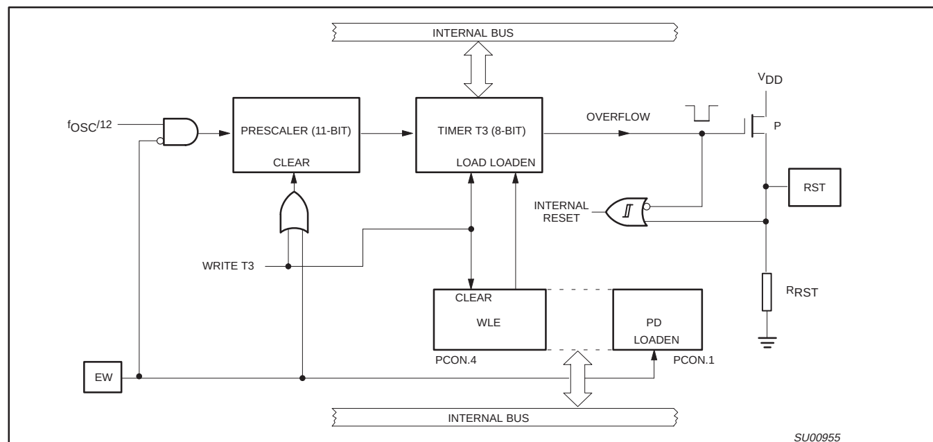
Figure 17. Watchdog Timer
