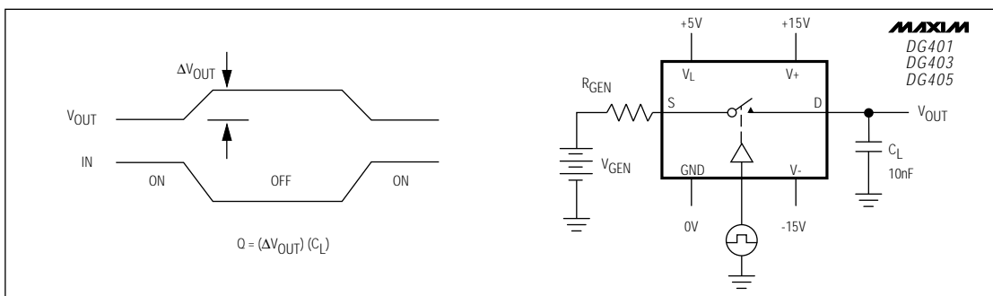
Figure 4. Charge Injection
