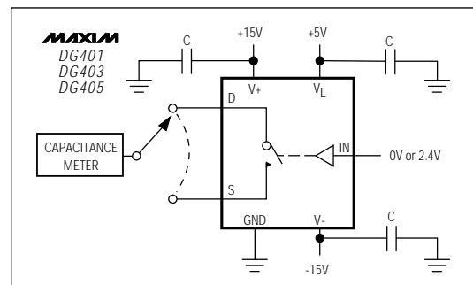
Figure 8. Channel-On Capacitance
