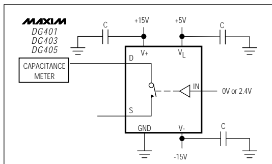
Figure 7. Channel-Off Capacitance
