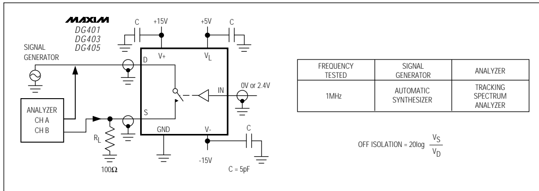
Figure 5. Off Isolation
