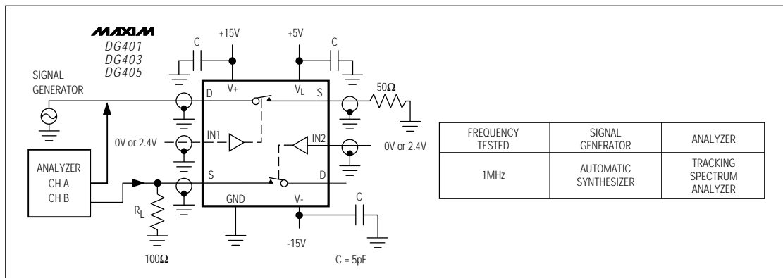
Figure 6. Crosstalk
