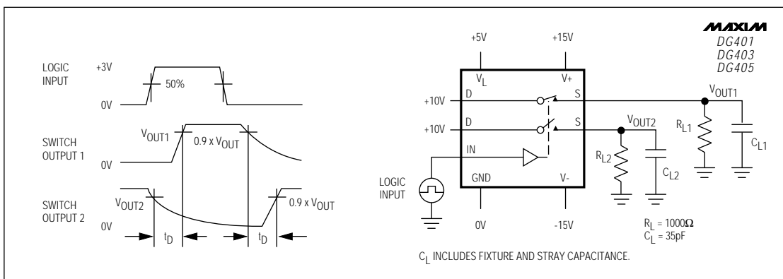
Figure 3. Break-Before-Make Interval
