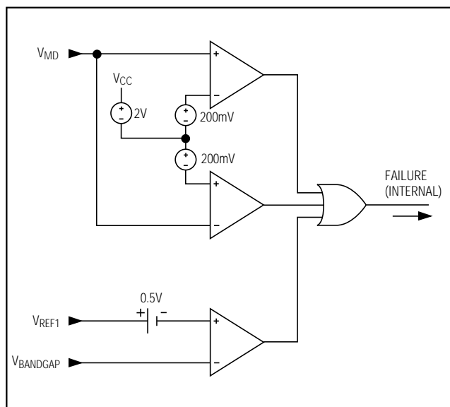
Figure 3. Failure-Detection Circuit (Simplified)
