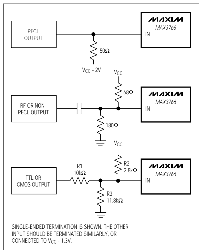
Figure 9. Input Terminations
