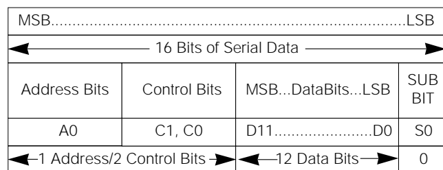
Figure 4. Serial-Data Format
