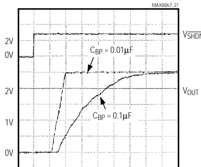
MAX886_EUK25 SHUTDOWN EXIT DELAY
