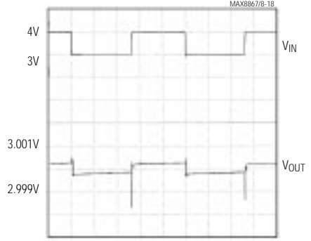
LINE-TRANSIENT RESPONSE
