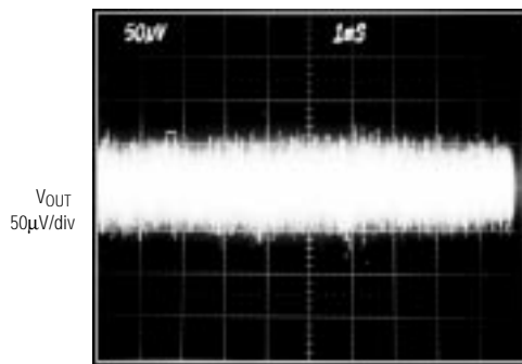
MAX886_EUK25 10Hz TO 100kHz OUTPUT NOISE
