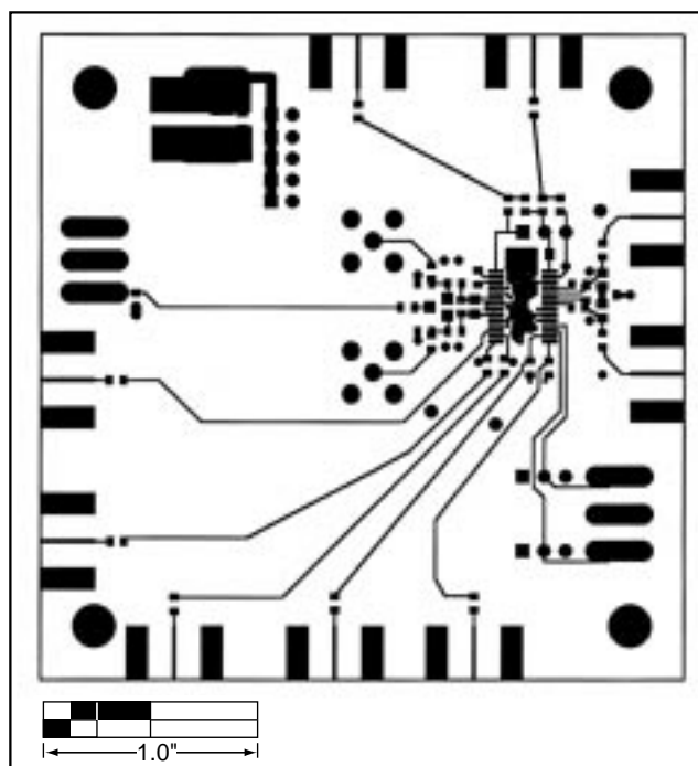
Figure 4. MAX2511EV Kit PC Board Layout—Component Side (layer 1)
