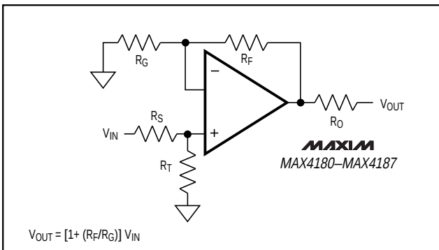
Figure 4b. Noninverting Gain Configuration
