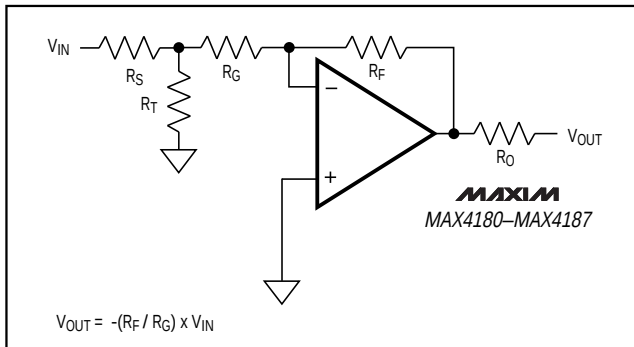
Figure 4a. Inverting Gain Configuration
