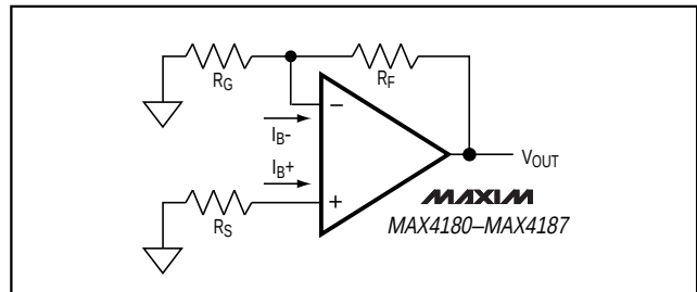
Figure 5. Output Offset Voltage
