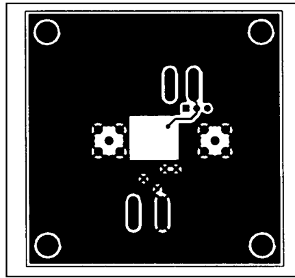
Figure 3c. SO-8 High-Speed EV Board Layout—Solder Side
