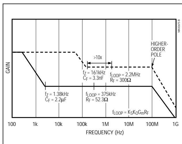
Figure 3. Loop-Filter Response
