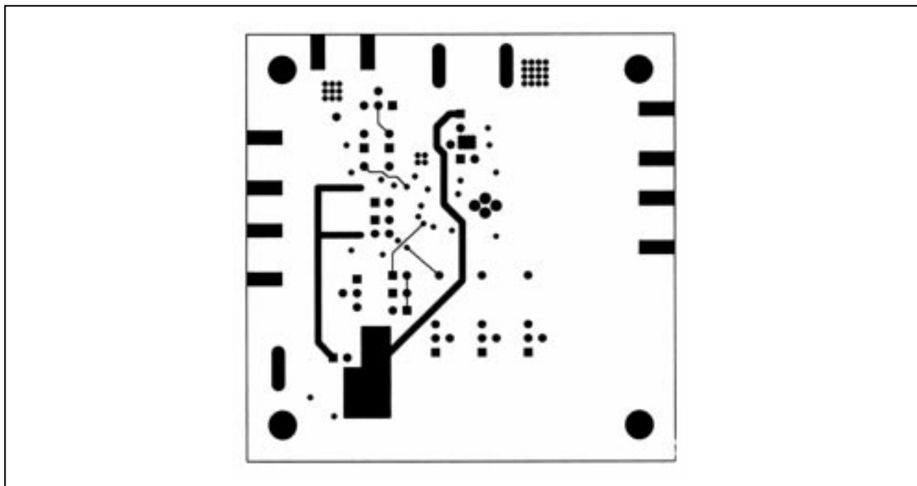
Figure 4. MAX3962 EV Kit PC Board Layout—Solder Side
