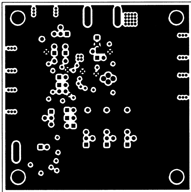
Figure 6. MAX3962 EV Kit PC Board Layout—Power Plane
