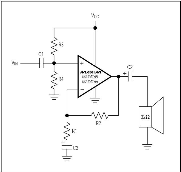
Typical Operating Circuit
