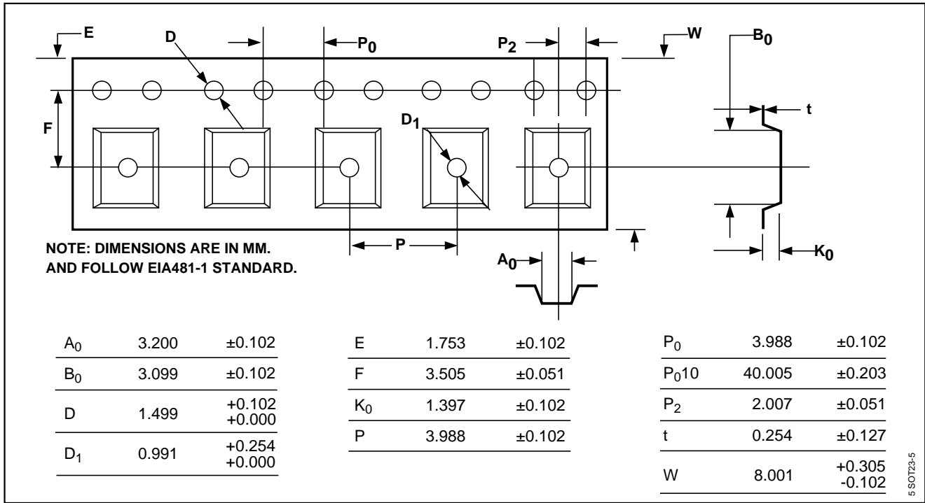
Tape-and-Reel Information
