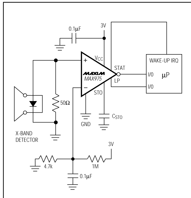
Figure 6. Toll-Tag Reader
