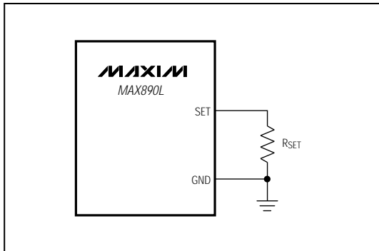
Figure 2. Setting the Current Limit
