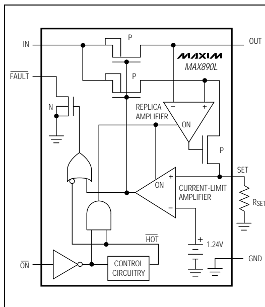
Figure 1. Functional Diagram
