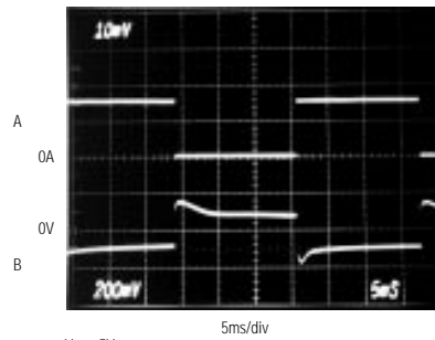
LOAD-TRANSIENT RESPONSE
