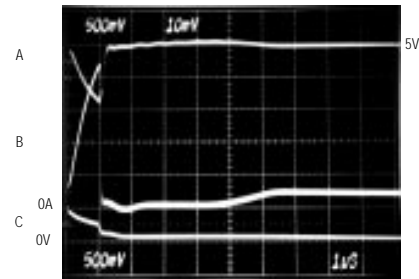
CURRENT-LIMIT RESPONSE ( R_L = 0.5\Omega )
