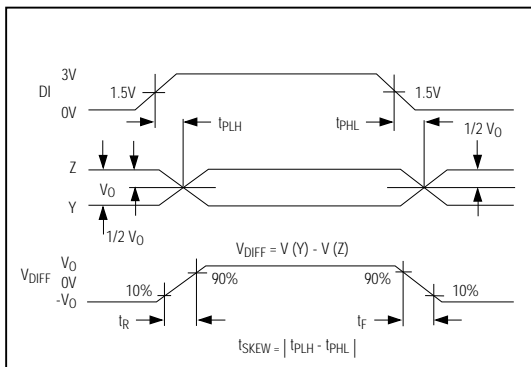
Figure 9. Driver Propagation Delays
