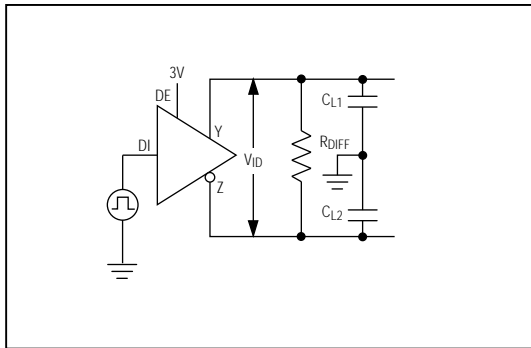
Figure 7. Driver Timing Test Circuit
