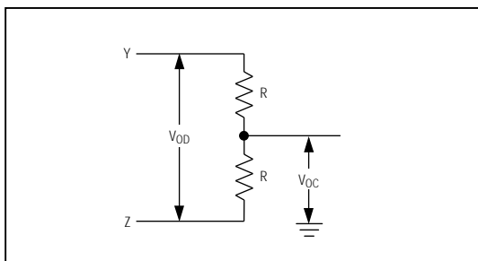
Figure 5. Driver DC Test Load
