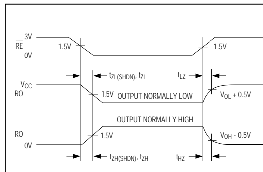
Figure 12. Receiver Enable and Disable Times (except MAX3081/MAX3084/MAX3087)
