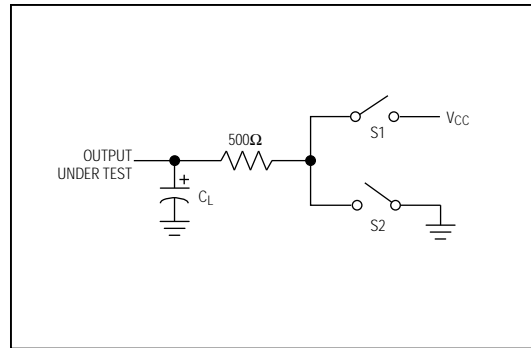
Figure 8. Driver Enable/Disable Timing Test Load
