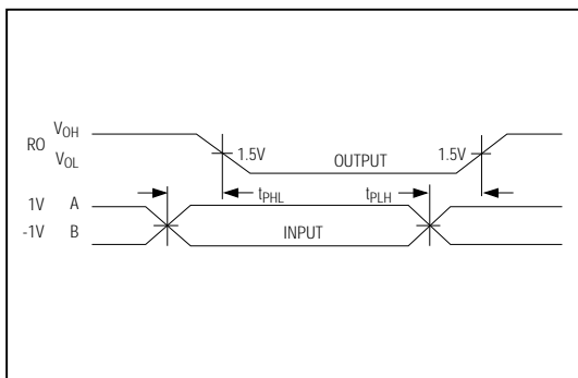
Figure 11. Receiver Propagation Delays
