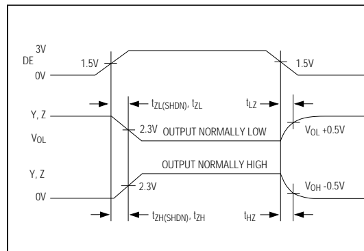
Figure 10. Driver Enable and Disable Times (except MAX3081/MAX3084/MAX3087)
