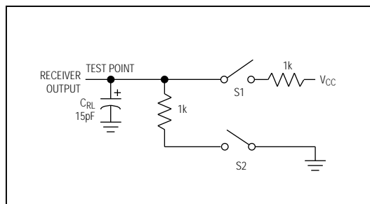
Figure 6. Receiver Enable/Disable Timing Test Load
