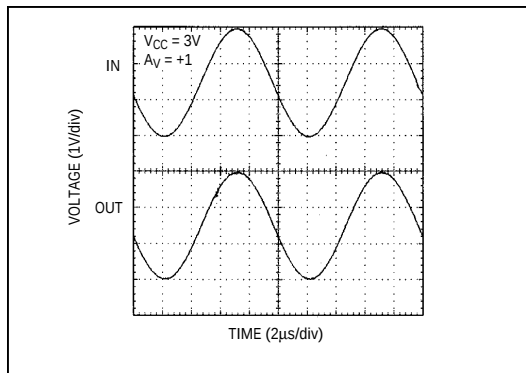
Figure 3. Rail-to-Rail Input /Output Voltage Range
