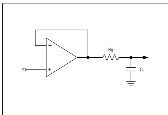
Figure 9. Capacitive-Load-Driving Circuit
