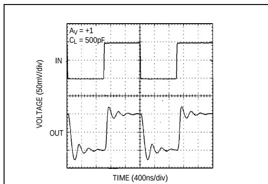
Figure 5. MAX4122/23/26/27/29 Small-Signal Transient Response with Capacitive Load
