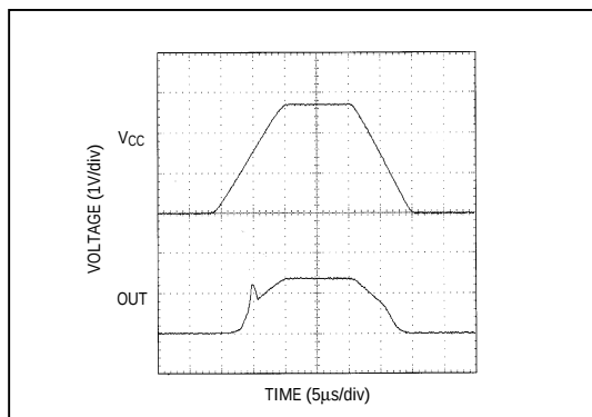
Figure 11. Power-Up Output Voltage
