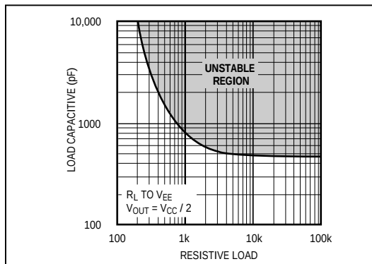
Figure 4. Capacitive-Load Stability
