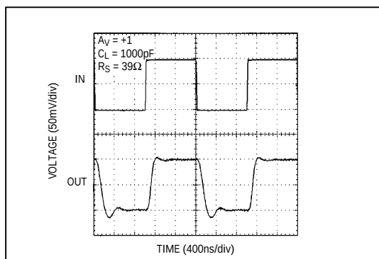
Figure 7. MAX4122/23/26/27/29 Transient Response to Capacitive Load with Isolation Resistor
