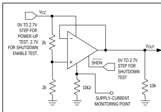
Figure 10. Power-Up/Shutdown Test Circuit
