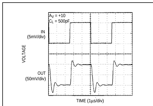
Figure 6. MAX4124/25/28 Small-Signal Transient Response with Capacitive Load
