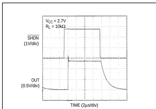
Figure 13. Shutdown Output Voltage
