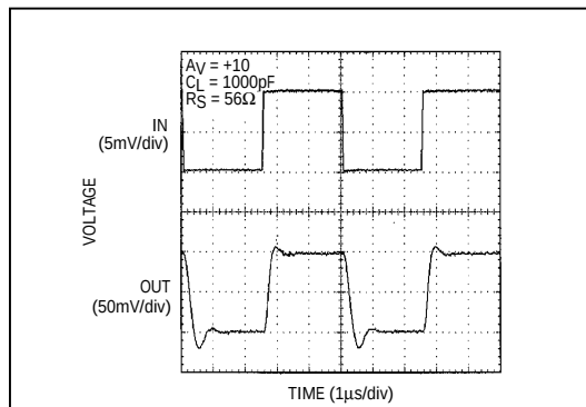
Figure 8. MAX4124/25/28 Transient Response to Capacitive Load with Isolation Resistor
