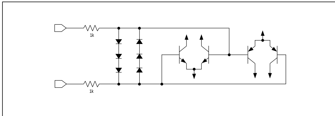
Figure 2. Input Protection Circuit
