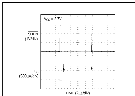
Figure 14. Shutdown Enable/Disable Supply Current
