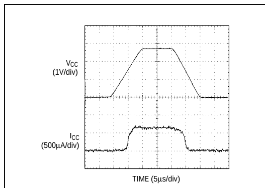
Figure 12. Power-Up Supply Current
