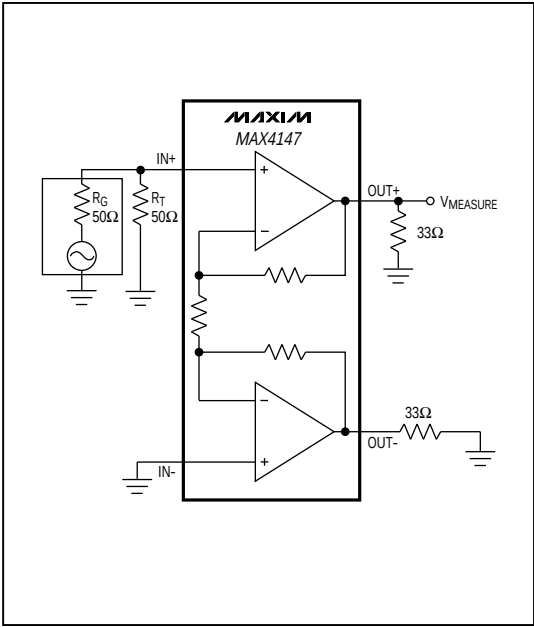
Figure 1. Single-Ended Distortion Setup
