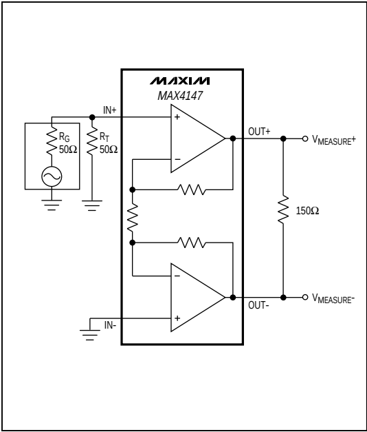
Figure 2. Differential Distortion Setup
