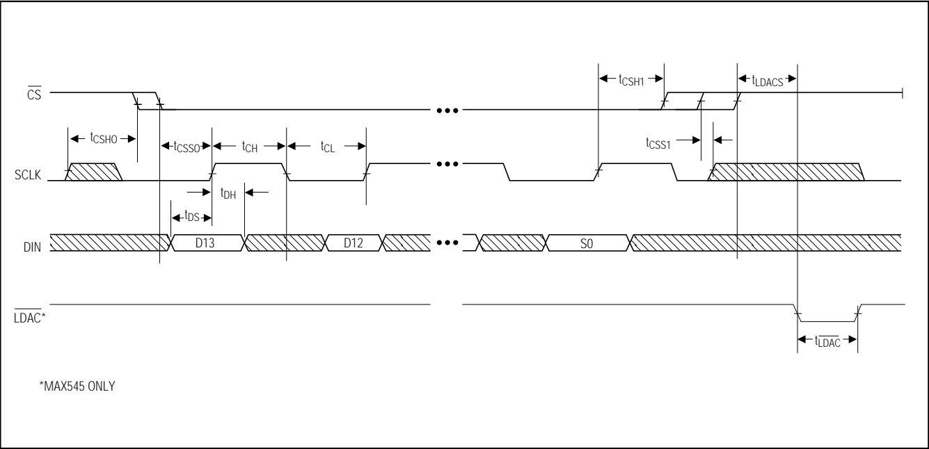
Figure 1. Timing Diagram
