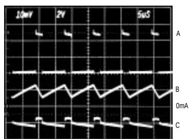
SWITCHING WAVEFORMS— CONTINUOUS CONDUCTION
