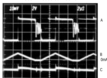
SWITCHING WAVEFORMS— DISCONTINUOUS CONDUCTION
