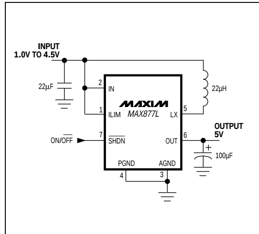
Figure 4. MAX877L Standard Application Circuit
