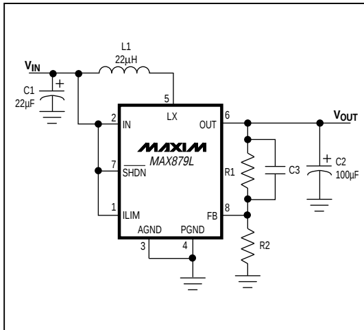
Figure 3. MAX879L Adjustable Voltage
