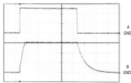
MAX878L START-UP TIME
