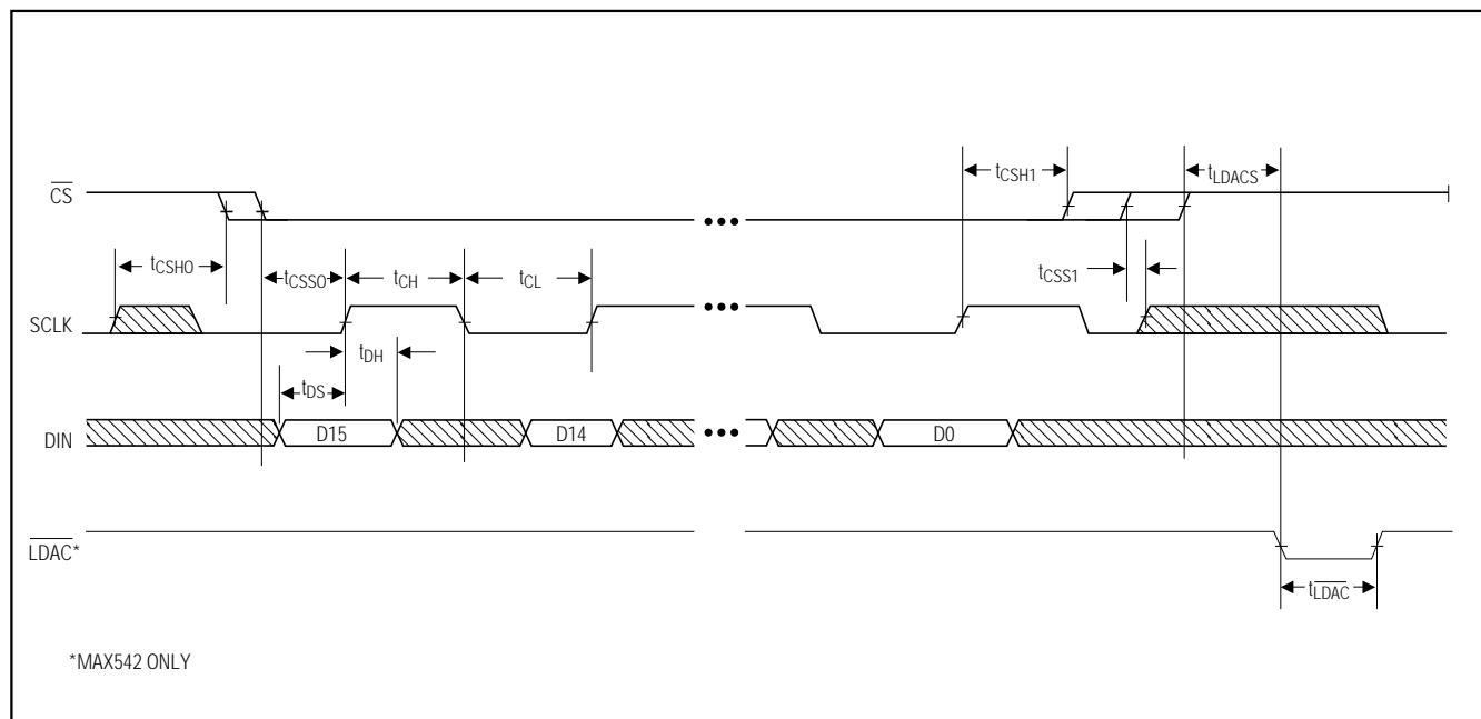
Figure 1. Timing Diagram
