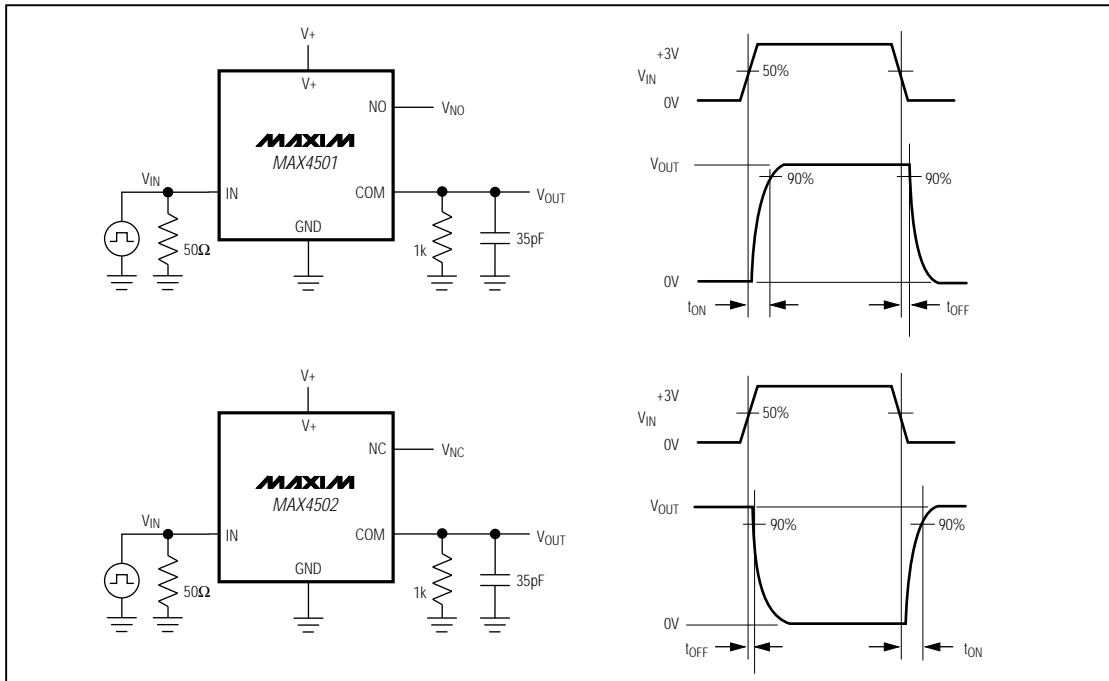
Figure 1. Switching Times
