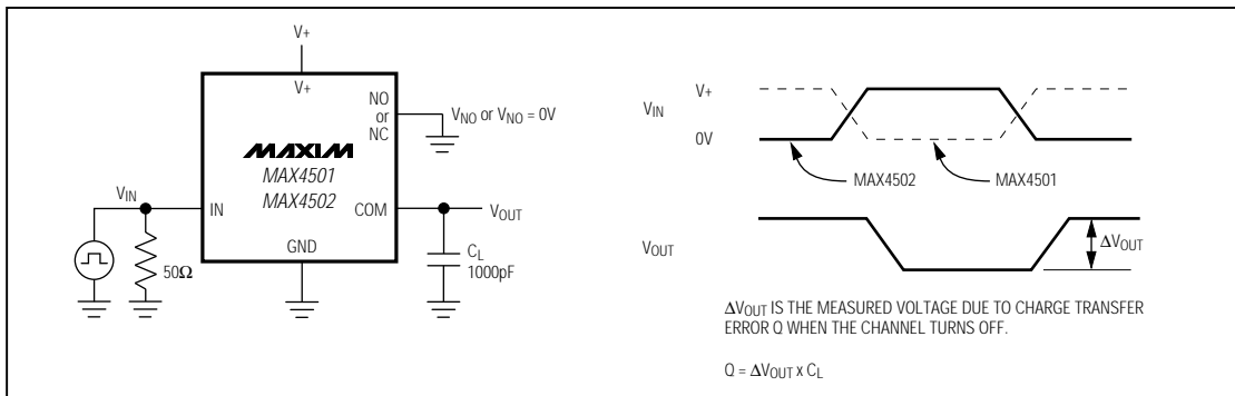
Figure 2. Charge Injection
