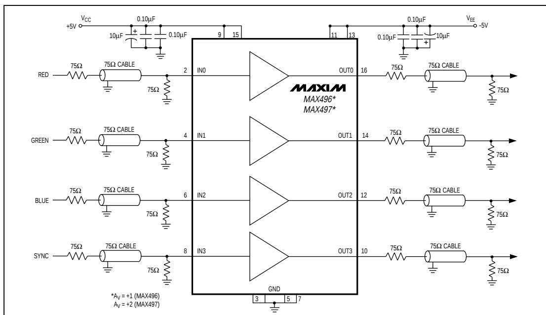
Figure 1. Typical Operating Circuit
