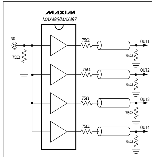
Figure 3. One-to-Four Distribution Amplifier
