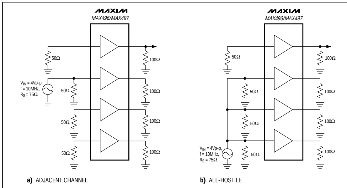
Figure 4. Crosstalk: a) Adjacent Channel; b) All-Hostile
