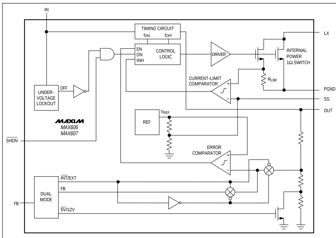
Figure 3. Functional Diagram
