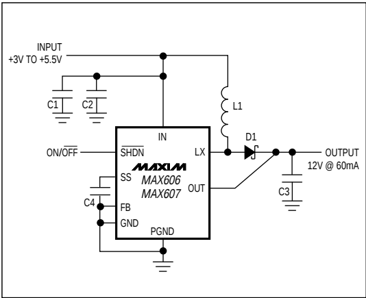
Figure 1. 12V Standard Application Circuit
