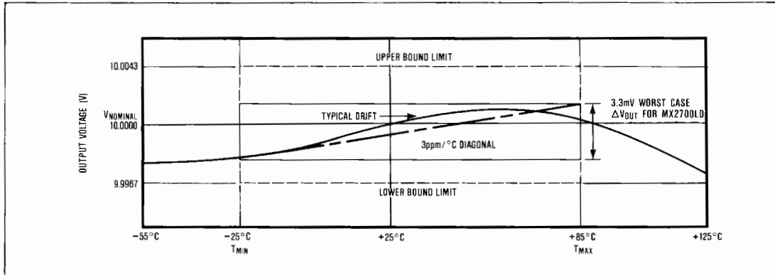
Figure 3. MX2700 Output Voltage Drift
