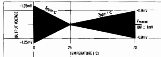
Figure 4a. MX2710K Output Voltage Drift
