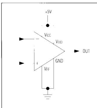
Figure 1B. Single +5V Supply, Common Ground
