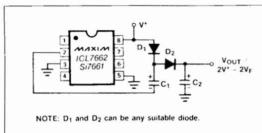
Figure 7. Positive Voltage Doubler
