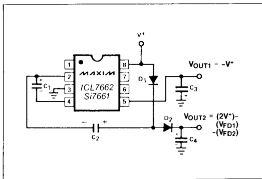
Figure 9. Combined Positive Multiplier and Negative Voltage Converter
