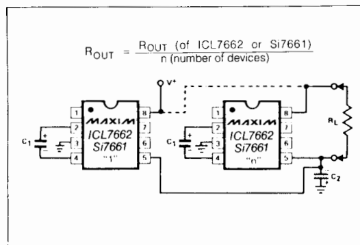
Figure 8. Paralleling ICL7662s to Reduce Output Resistance
