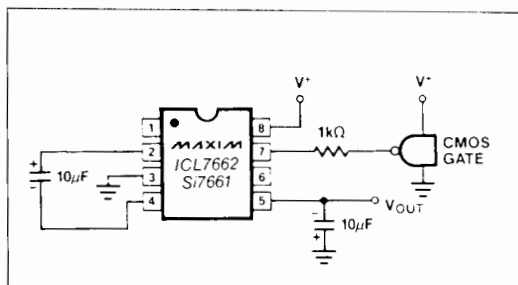
Figure 4. External Clocking
