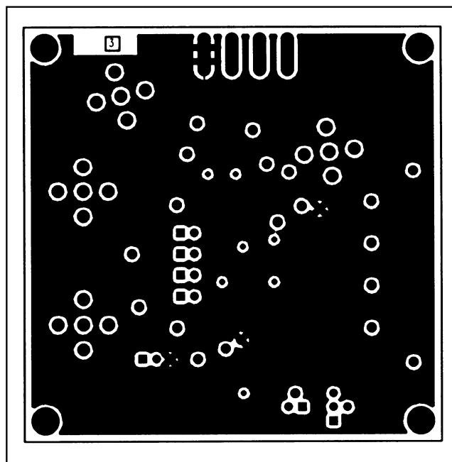
Figure 5. MAX2450 EV Kit PC Board Layout—Power Plane
