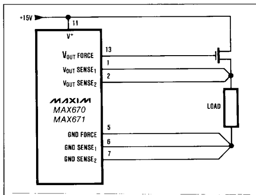
Figure 3. FET Source Follower
