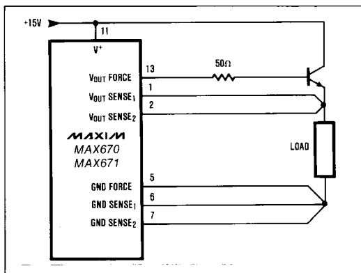
Figure 2. NPN Emitter Follower
