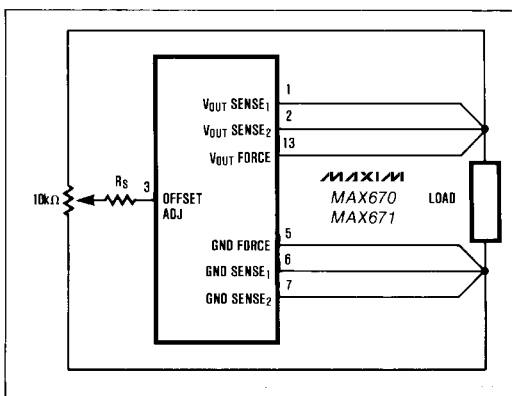
Figure 9. MAX670/671 Improved TC Independent Trim Adjustment
