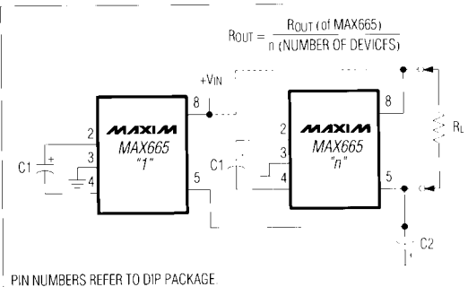
Figure 4. Paralleling MAX665s to Reduce Output Resistance
