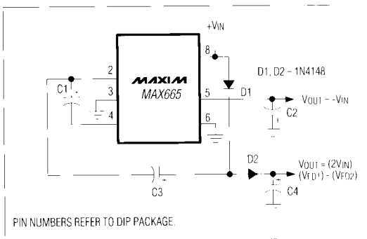
Figure 5. Combined Positive Multiplier and Negative Converter
