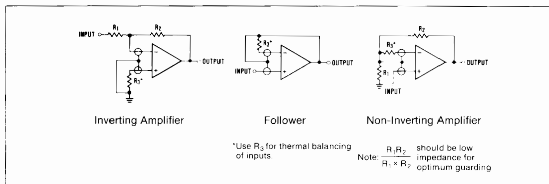
Figure 4. Input Guard Connections
