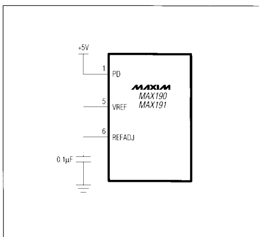
Figure 18a. Internal-Compensation Mode Circuit
