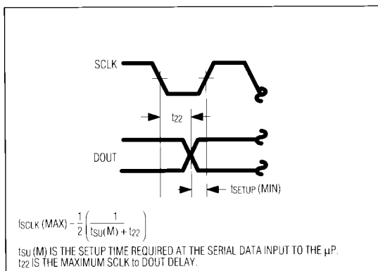
Figure 12. f_{\text{SCLK}}(\text{MAX}) is limited by the setup time required by the serial data input to the \mu\text{P} .
