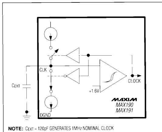
Figure 5. Internal Clock Circuit
