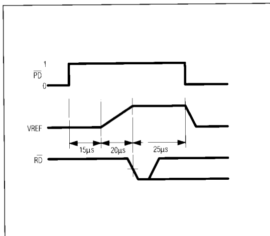
Figure 18b. Low Average-Power Mode Operation (Internal Compensation)
