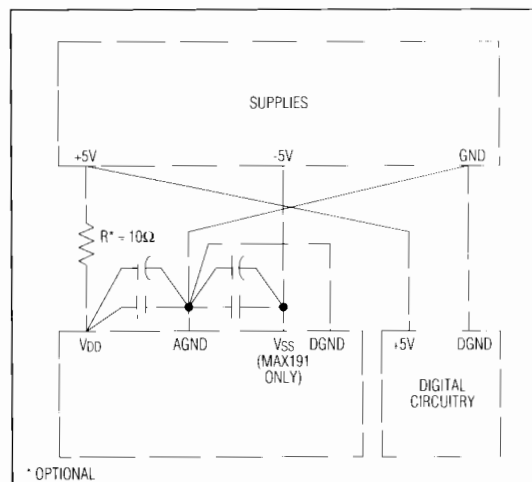
Figure 23. Power-Supply Grounding Connection
