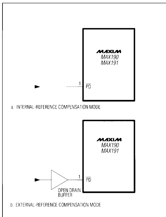
Figure 17. Drive Circuits for \overline{\text{PD}} pin
