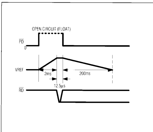
Figure 19b. Low Average-Power Mode Operation (External Compensation)
