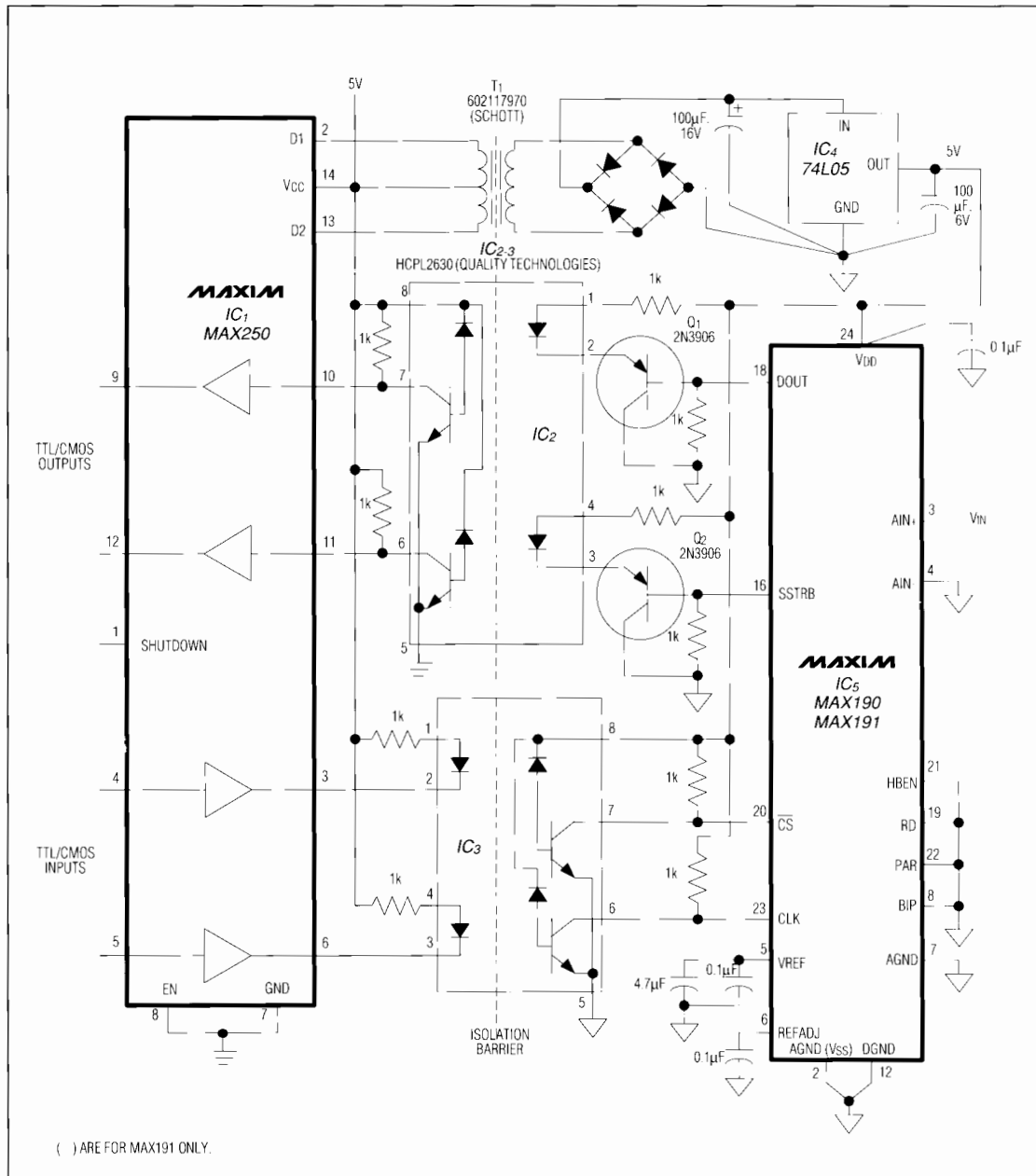
Figure 24. Isolated Data-Acquisition Circuit
