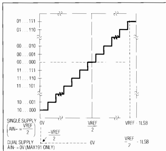
Figure 22. MAX190/MAX191 Bipolar Transfer Function
