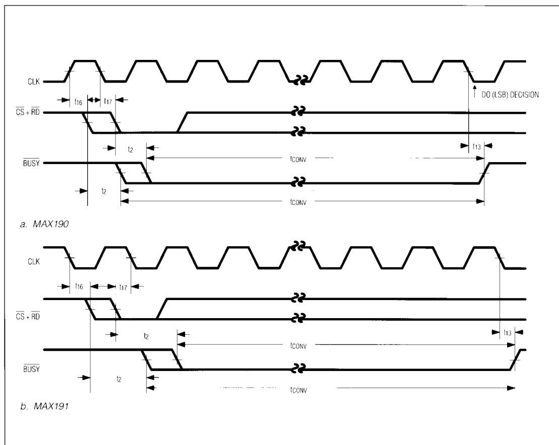
Figure 6. CS, RD, and CLK Synchronous Operation
