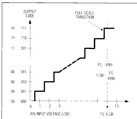
Figure 20. MAX190/MAX191 Unipolar Transfer Function
