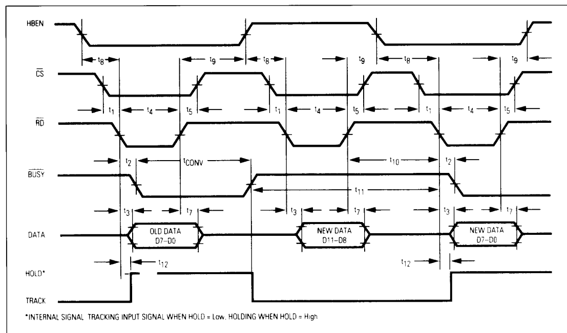
Figure 8. ROM Mode, 2-Byte Read Data-Bus Status
