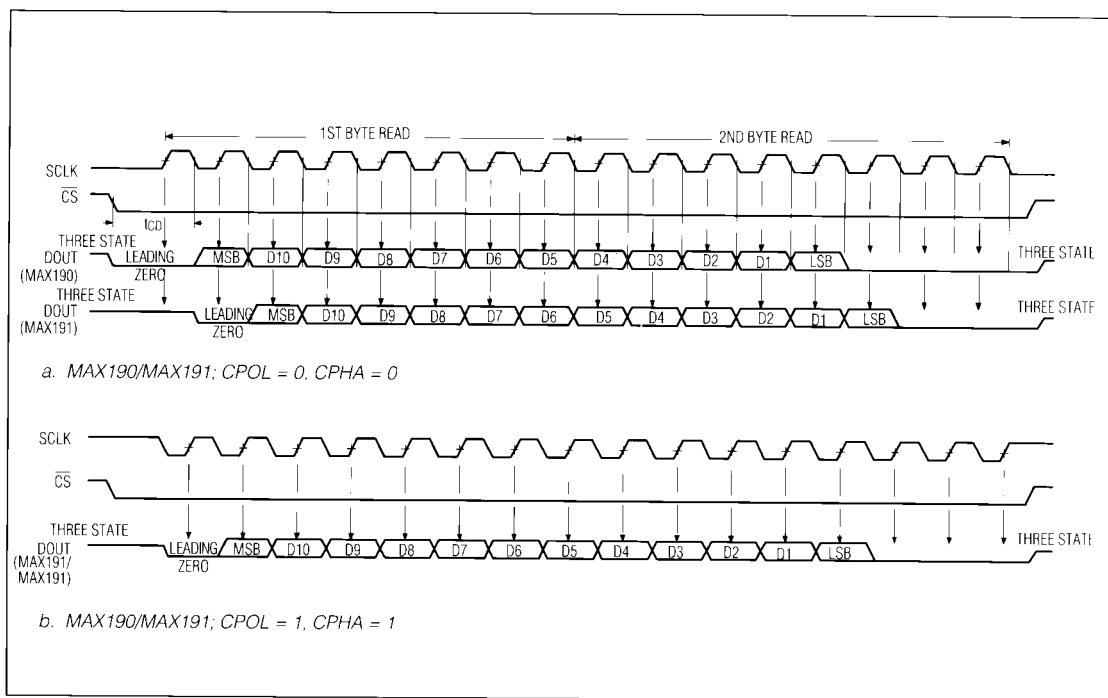
Figure 14. SPI/Microwire Serial-Interface Timing
