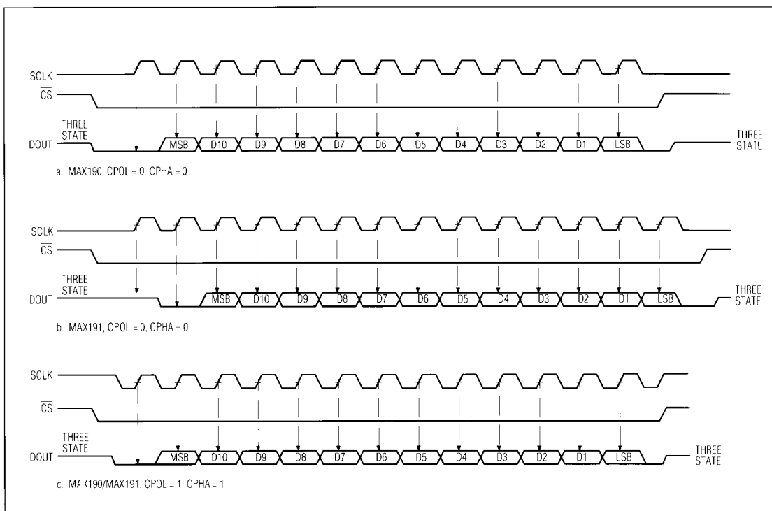
Figure 15. QSPI Serial-Interface Timing
