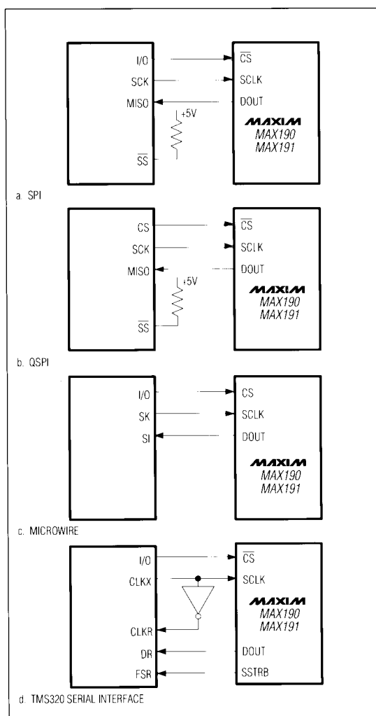
Figure 13. Common Serial-Interface Connections to the MAX190/MAX191
