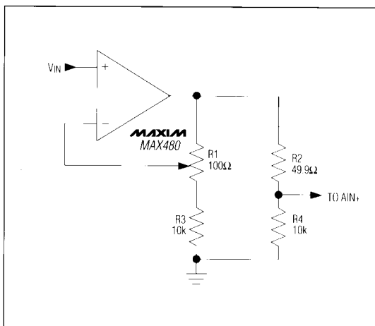
Figure 21a. Trim Circuit for Gain ( \pm 0.5\% )
