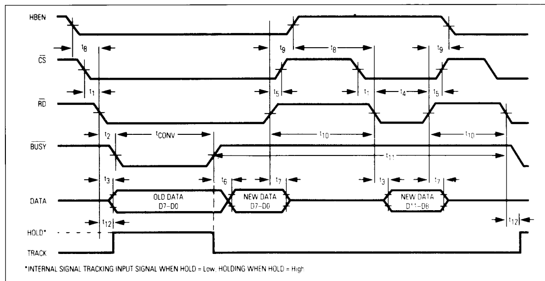
Figure 7. Slow-Memory Mode, 2-Byte Read Data-Bus Status
