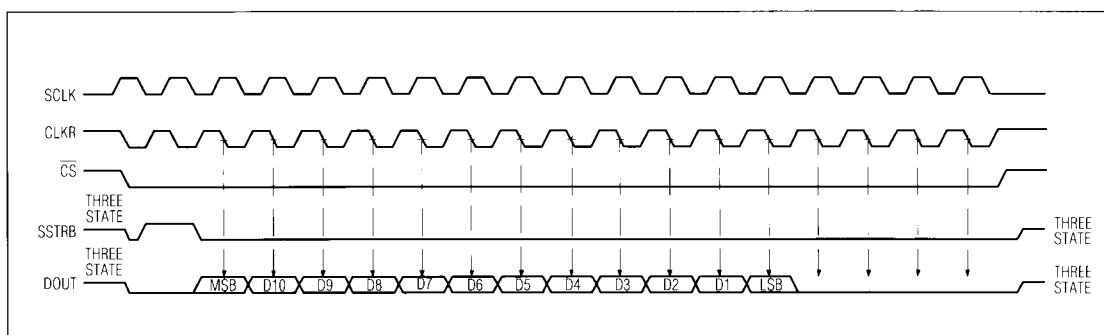
Figure 16. MAX190/MAX191 TMS320 Interface Timing
