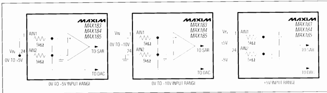
Figure 15. Analog Input Range Configurations
