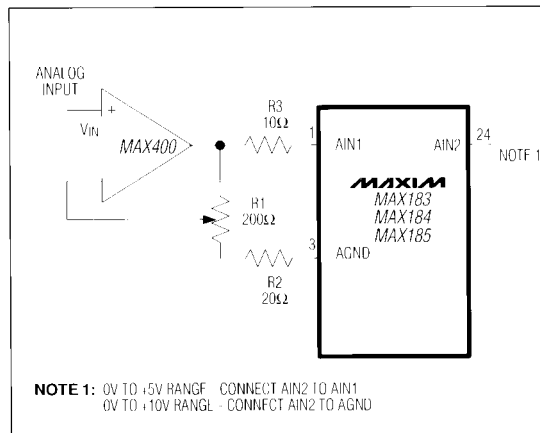
Figure 18. Unipolar Operation with Gain Adjust
