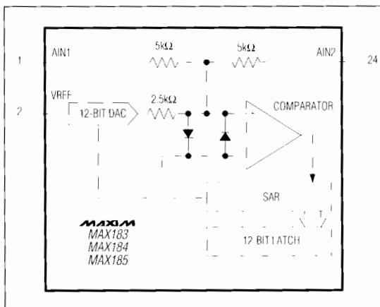
Figure 4. MAX183/184/185 AIN Inputs
