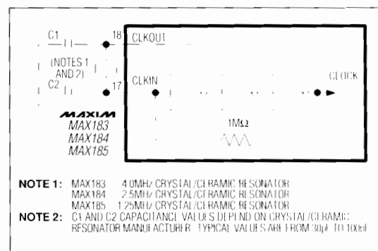
Figure 6. MAX183/184/185 Internal Clock Circuit
