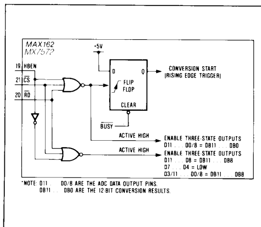
Figure 9. Logic Equivalent for RD, CS and HBEN Inputs
