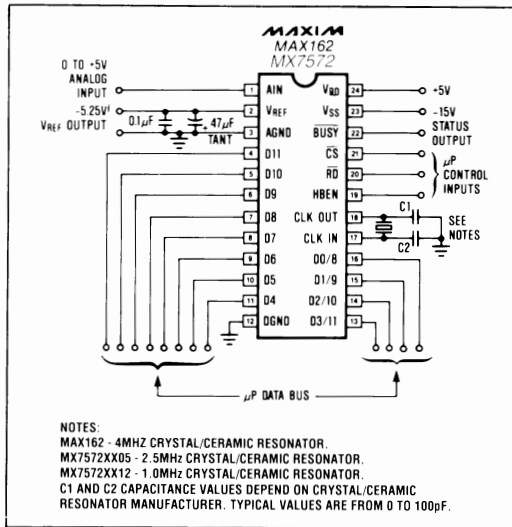
Figure 3. MAX162/MX7572 Operational Diagram
