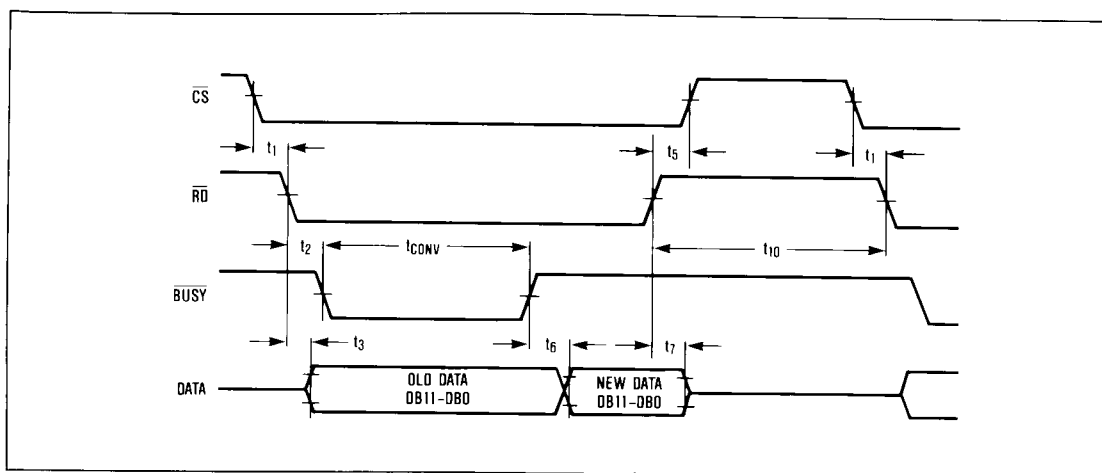
Figure 10. Slow Memory Mode, Parallel Read Timing Diagram
