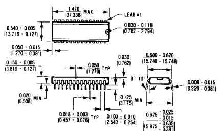
28 Lead Plastic DIP (PI)
