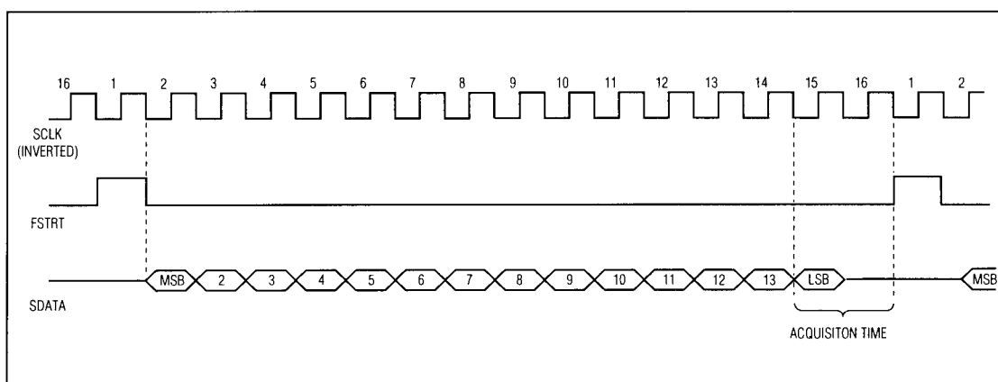
Figure 2. MAX121 EV Kit Continuous-Conversion Mode Timing
