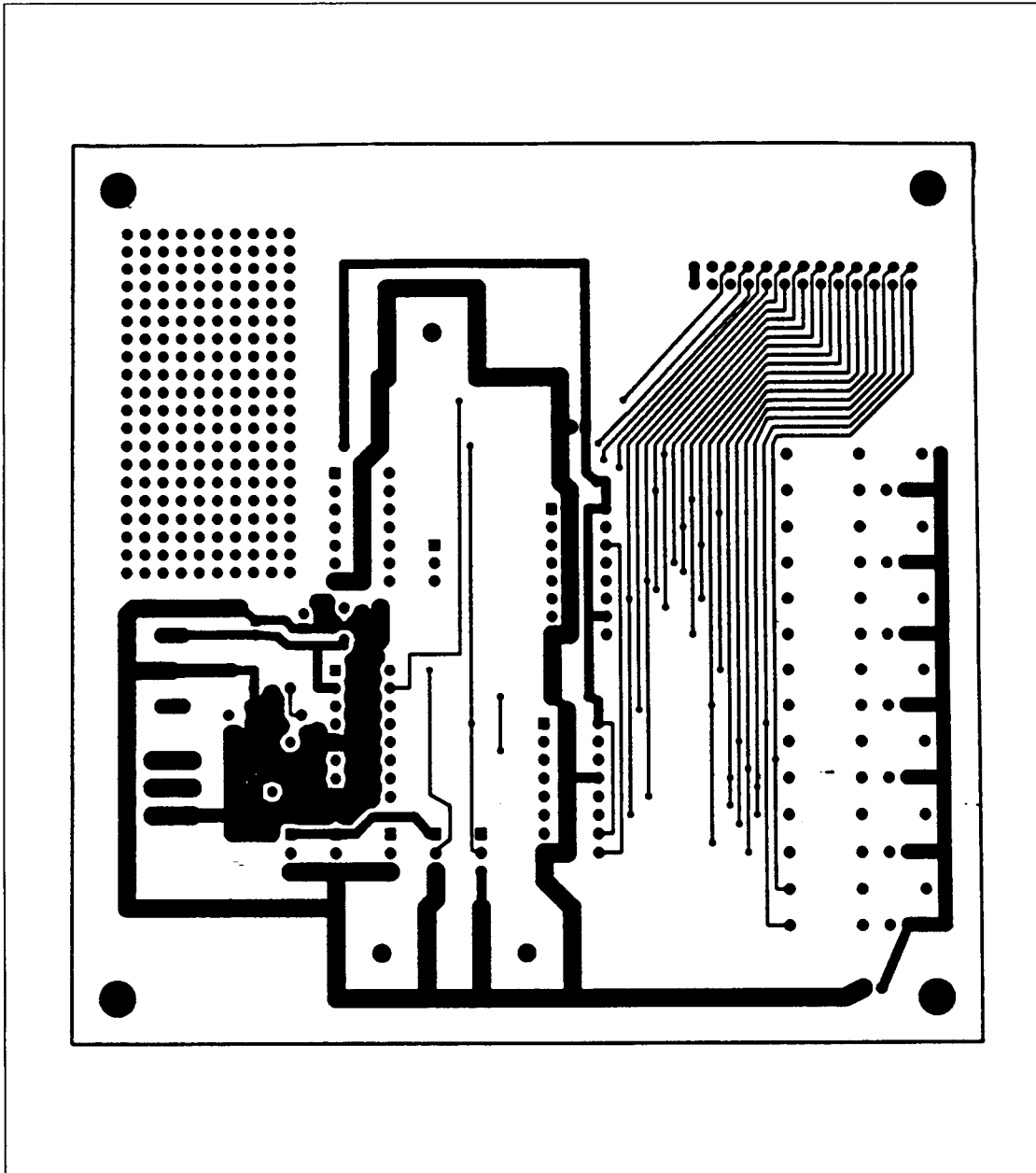
Figure 5. MAX121 EV Kit Component-Side Layout
