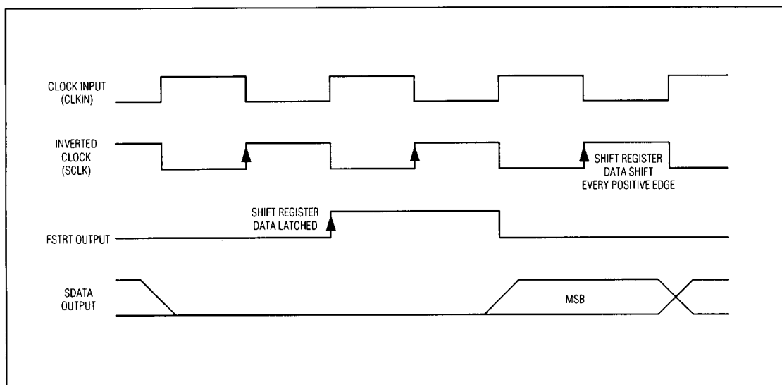
Figure 1. MAX121 Conversion Start
