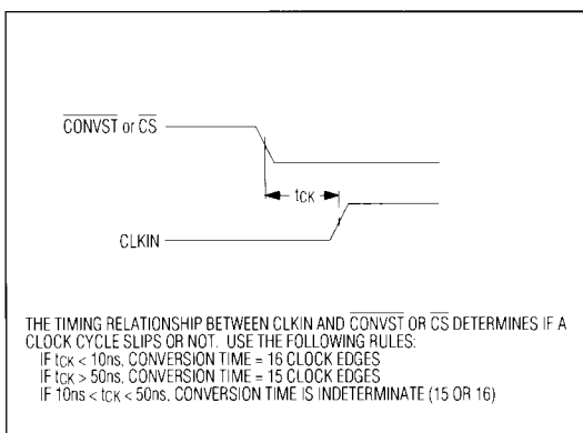
Figure 10. Clock and Control Synchronization
