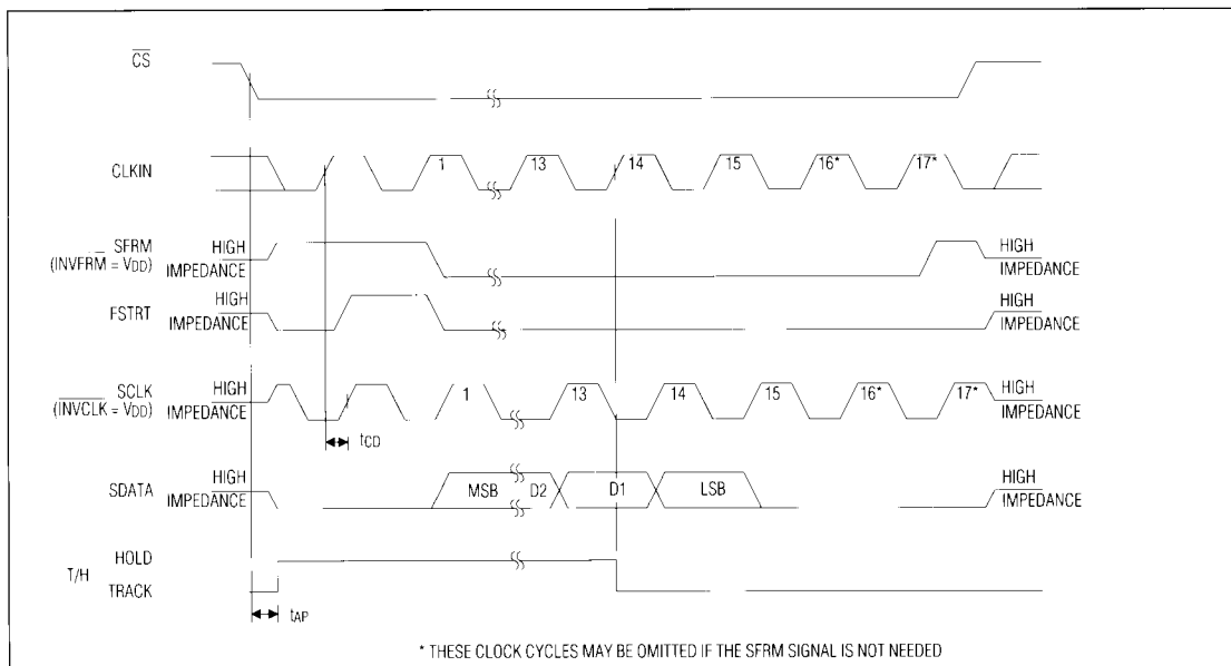
Figure 8. \overline{CS} Controls Conversion Starts (Mode 2)
