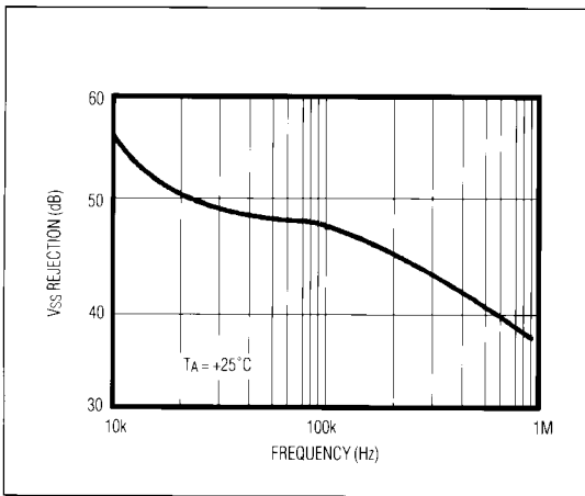
Figure 27. VSS Power-Supply Rejection vs. Frequency
