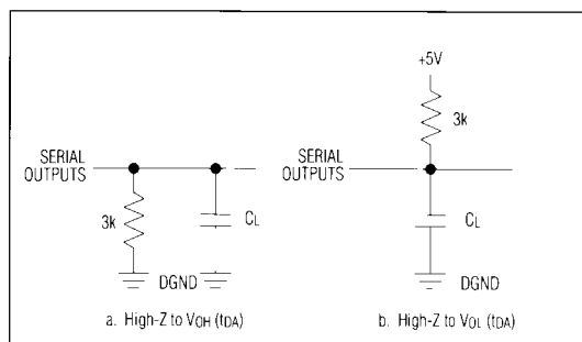
Figure 4. Load Circuits for Data-Access Time
