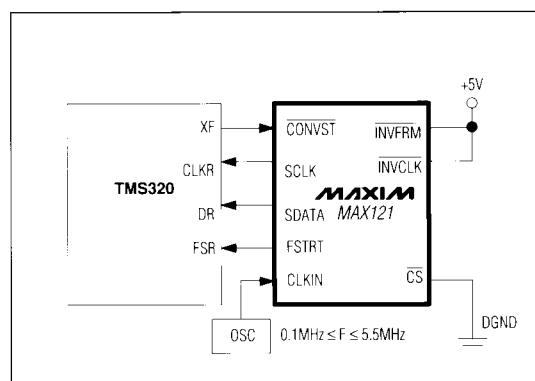
Figure 20. TMS320 High-Speed Serial-Interface Circuit
