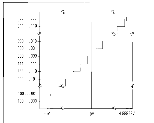
Figure 31. Bipolar Transfer Function
