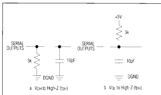
Figure 5. Load Circuits for Data-Hold Time
