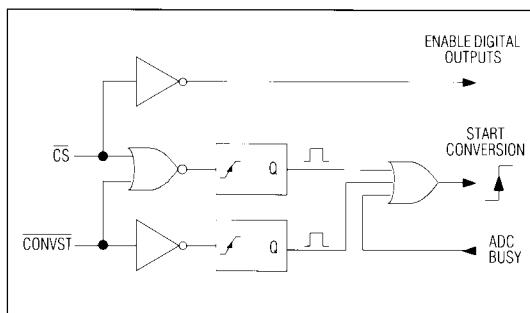
Figure 6. Conversion Control Logic
