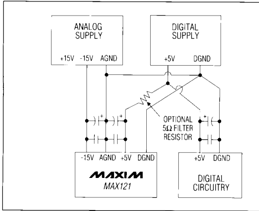
Figure 26. Power-Supply Grounding
