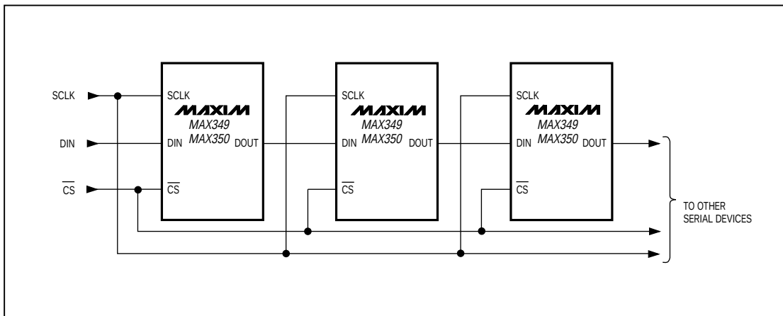
Figure 5. Daisy-Chained Connection
