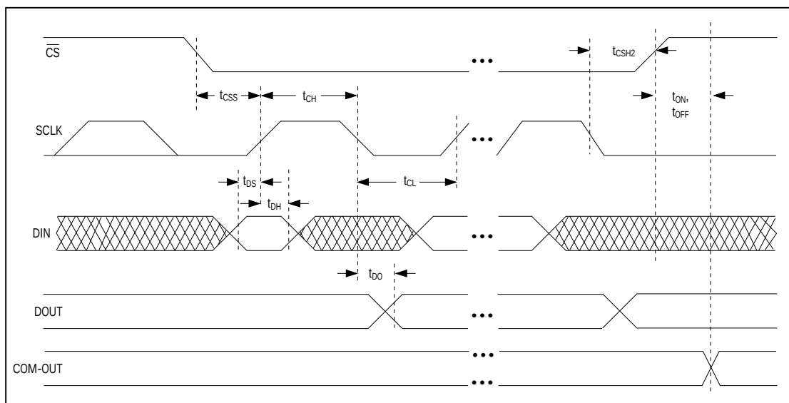
Figure 1. Timing Diagram
