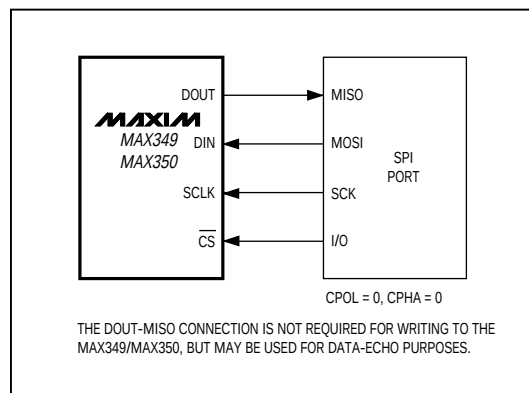
Figure 4. Connections for SPI and QSPI
