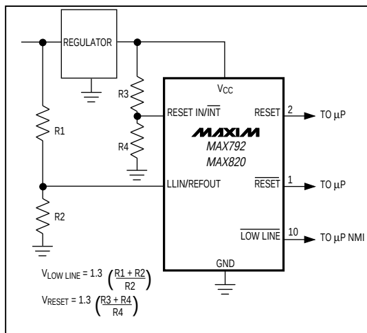
Figure 4c. Alternative connection for external programming mode
