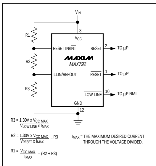
Figure 4b. Connection for External Threshold Programming Mode
