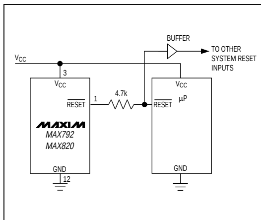
Figure 12. Interfacing to \mu\text{Ps} with Bidirectional RESET Pins
