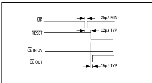
Figure 2. Manual-Reset Timing Diagram
