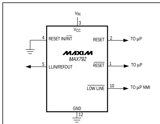
Figure 4a. Connection for Internal Threshold Mode
