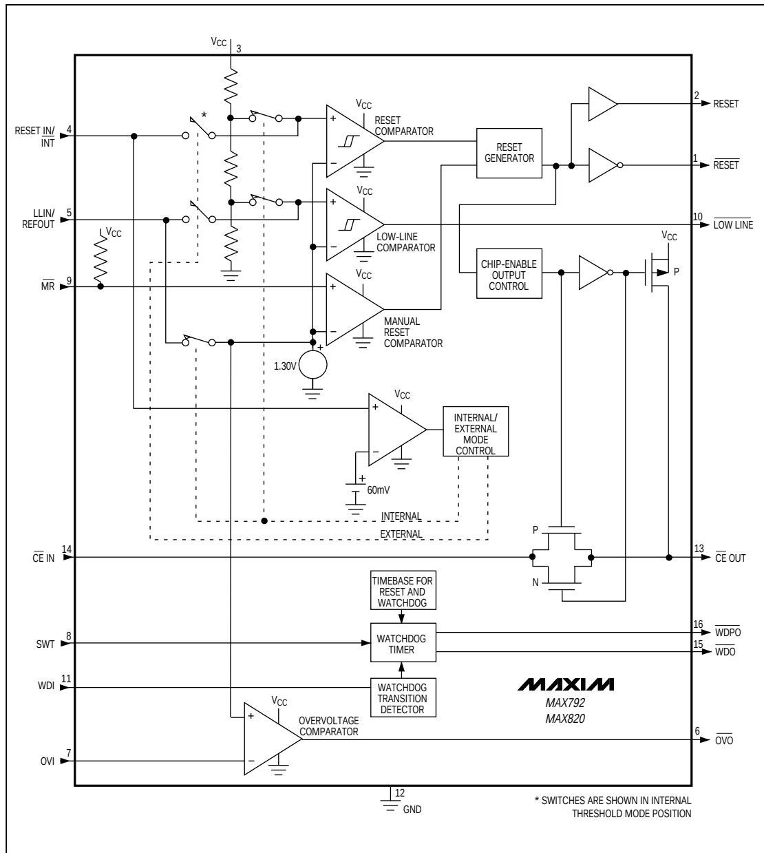
Figure 1. Block Diagram
