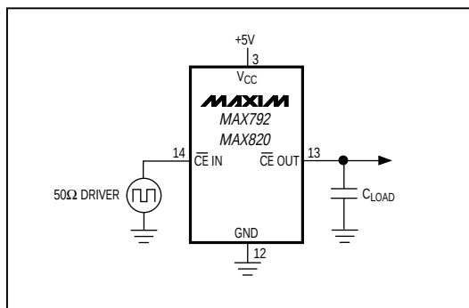
Figure 10. CE Propagation Delay Test Circuit
