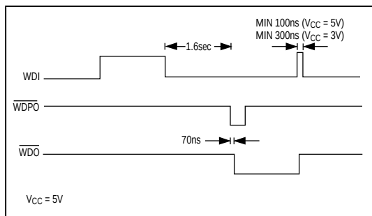
Figure 7. WDI, WDO and WDPO Timing Diagram
