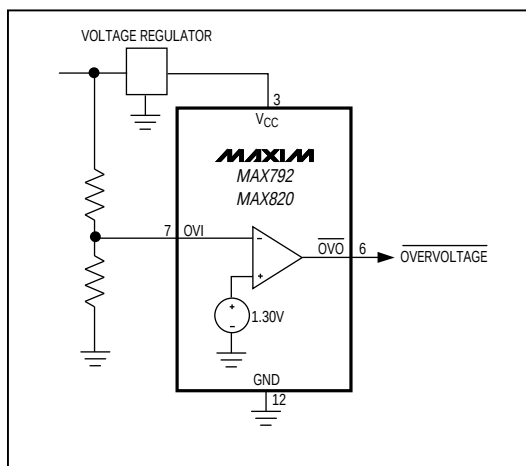
Figure 6. Detecting an Overvoltage Condition
