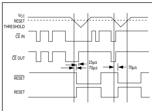
Figure 9. Reset and Chip-Enable Timing
