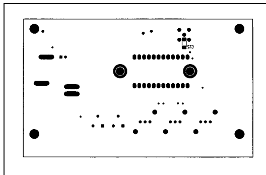
Figure 3. MAX445 EV Kit Component Placement Guide—Solder Side
