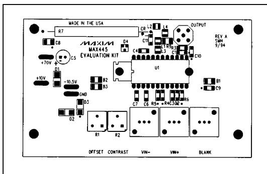
Figure 2. MAX445 EV Kit Component Placement Guide—Component Side
