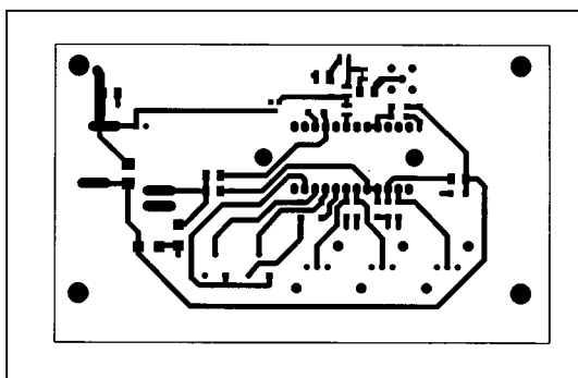
Figure 4. MAX445 EV Kit PC Board Layout—Component Side
