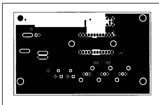
Figure 5. MAX445 EV Kit PC Board Layout—Solder Side
