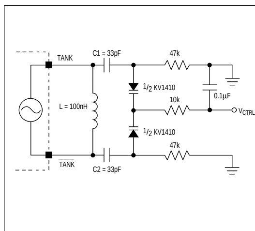
Figure 4. Typical Resonant Tank Circuit
