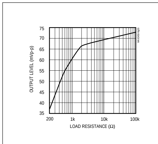
Figure 3. Modulator Output Level vs. Load Resistance
